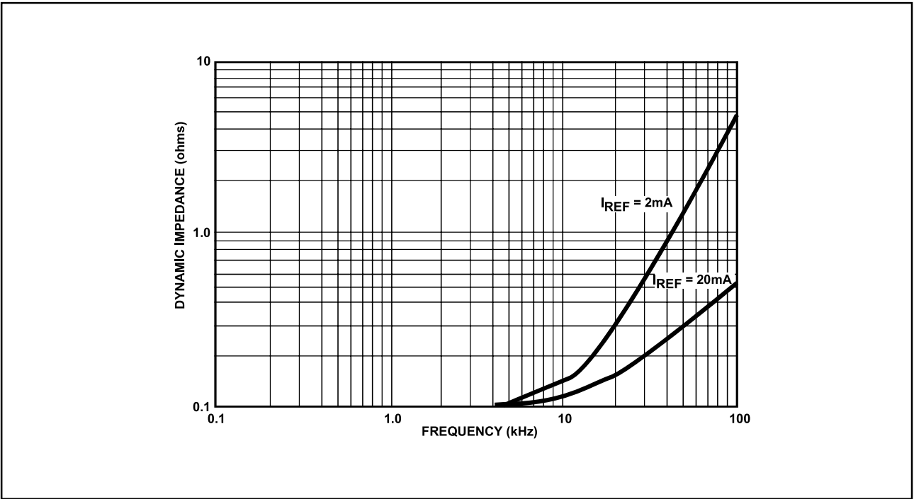
Fig.3 Dynamic impedance
