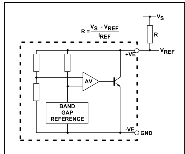
Fig.2 Circuit diagram
