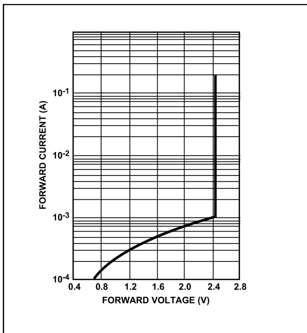
Fig.4 Forward characteristic
