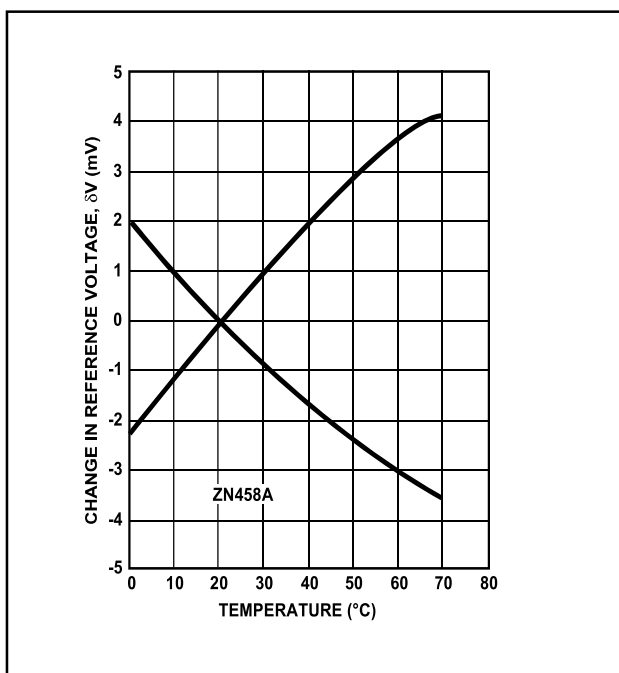
Fig.6 Temperature characteristic (typical)
