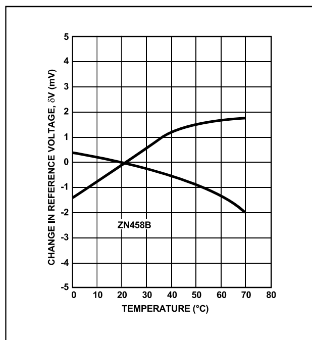
Fig.7 Temperature characteristic (typical)
