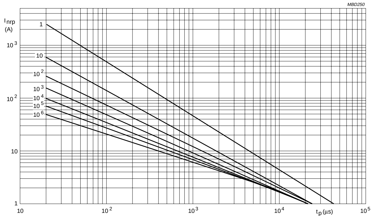
Fig.28 Maximum applicable transient current as a function of pulse duration, 385 V to 550 V (RMS); 2322 594 series.
