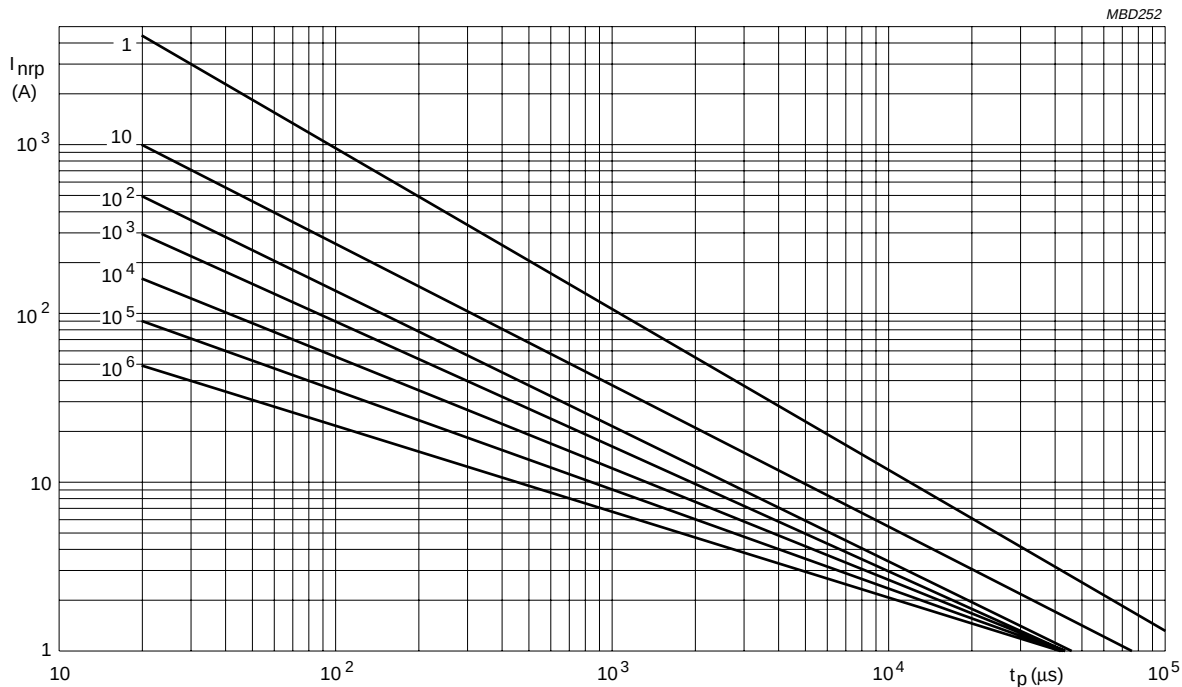
Fig.30 Maximum applicable transient current as a function of pulse duration, 50 V to 320 V (RMS); 2322 595 series.
