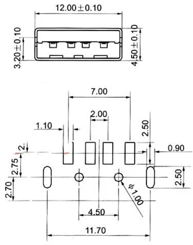
PCB LAYOUT
