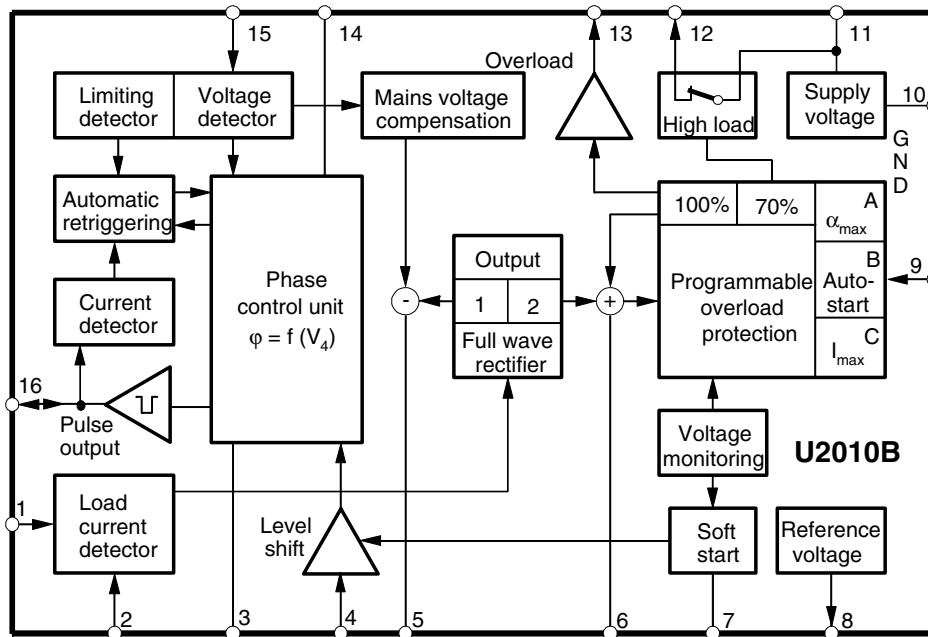
Figure 1-1. Block Diagram
