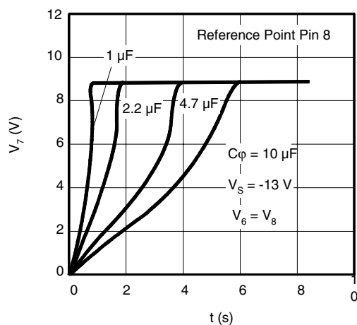
Figure 7-5. Soft-start Characteristic
