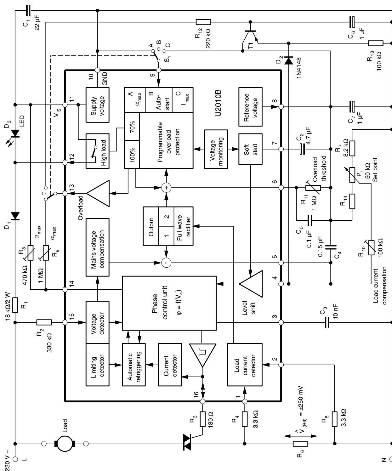
Figure 7-15. Application Circuit
