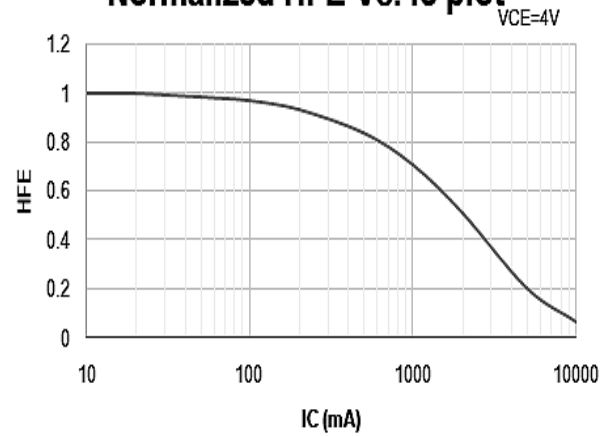
Normalized HFE Vs. Ic plot
