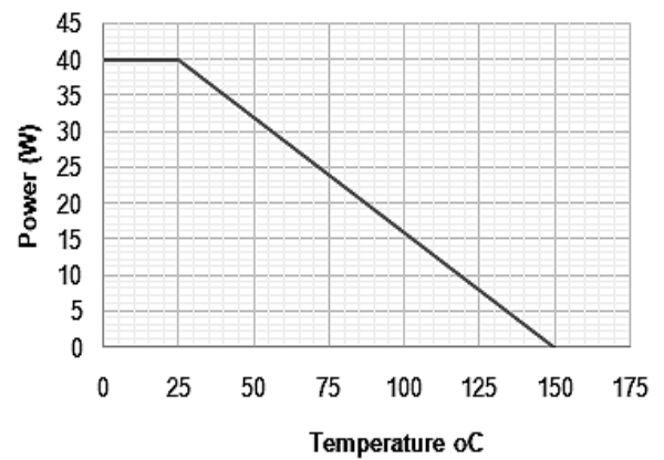
Power dissipation Chart
