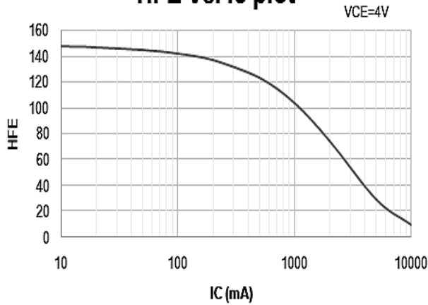
HFE Vs. Ic plot
