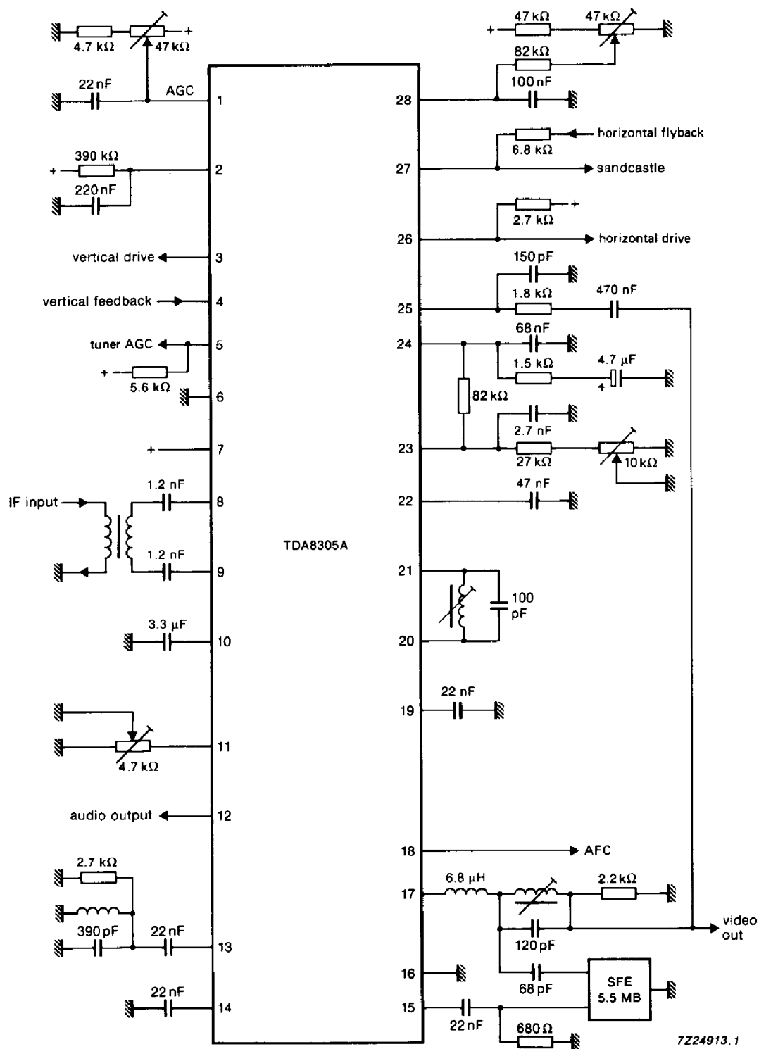
Fig.11 Application diagram.
