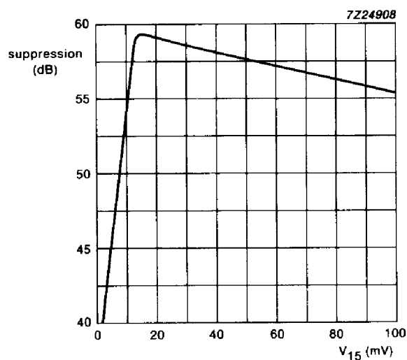
Fig.7 AM suppression.
