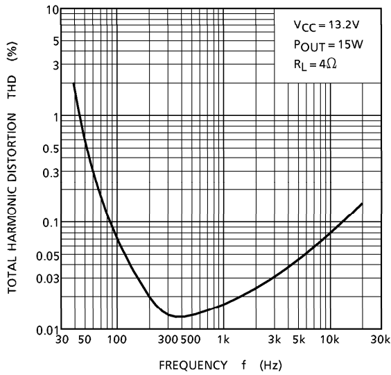
THD - f
