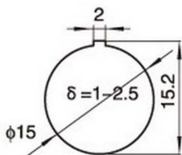
Panel Opening
