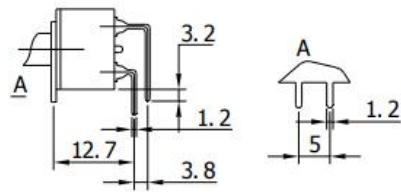
PC-H terminal(3)
