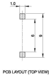
PCB LAYOUT (TOP VIEW)
