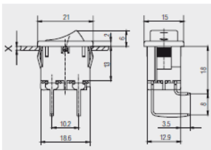
PCB terminal angled to terminal side 1
