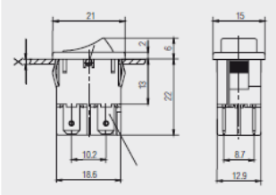
Quick-connect terminal 4.8
