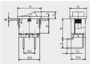
PCB terminal angled to terminal side 2
