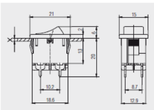
PCB terminal
