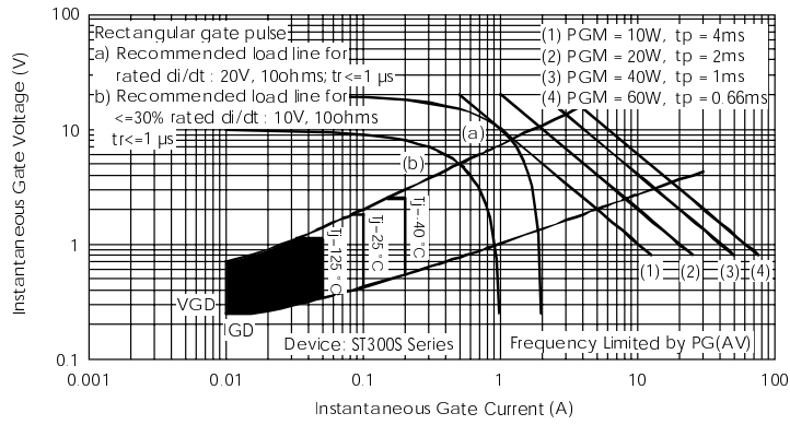
Fig. 9 - Gate Characteristics
