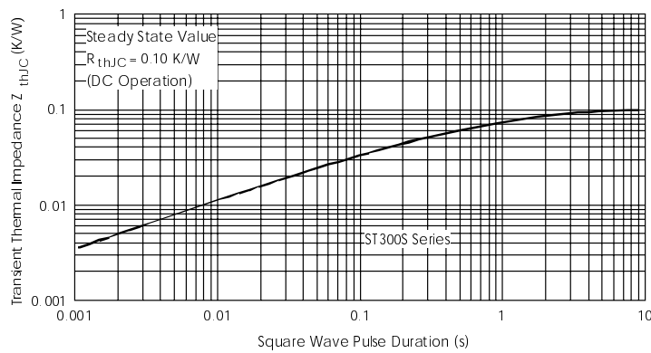
Fig. 8 - Thermal Impedance Z_{thJC} Characteristic
