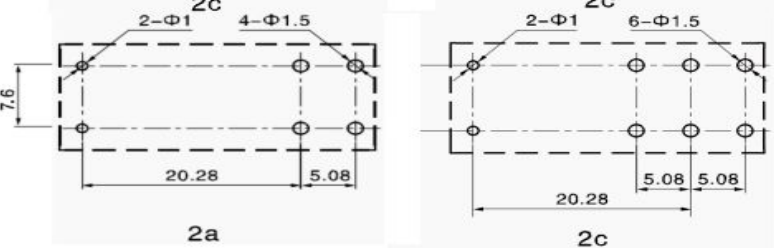
安装孔尺寸图(底视图) P. C. B. Layout (bottom view)
