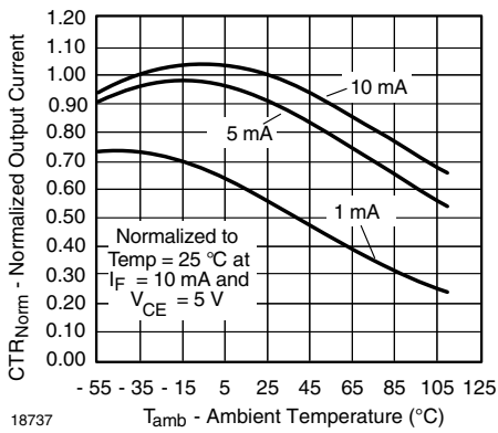
Figure 9. Normalized CTR vs. Temperature
