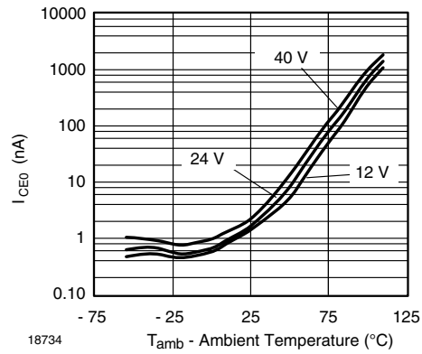
Figure 6. Collector to Emitter Dark Current vs. Ambient Temperature
