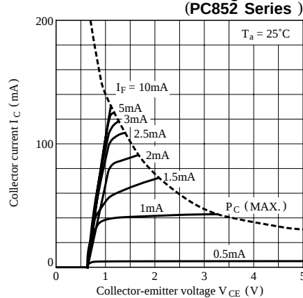
Fig. 6-a Collector Current vs. Collector-emitter Voltage
