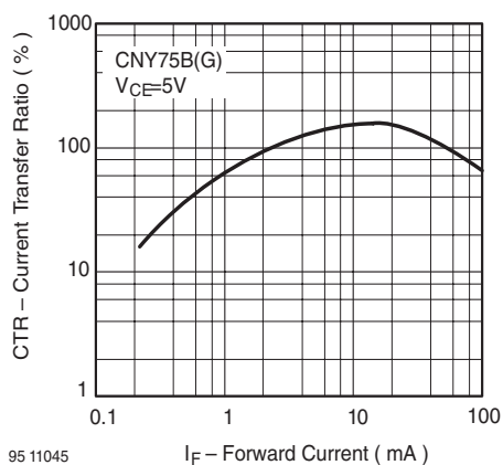
Figure 17. Current Transfer Ratio vs. Forward Current
