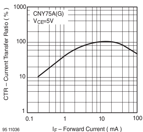
Figure 16. Current Transfer Ratio vs. Forward Current
