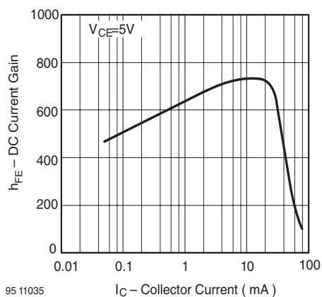
Figure 15. DC Current Gain vs. Collector Current
