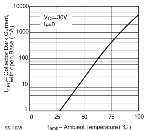
Figure 6. Collector Dark Current vs. Ambient Temperature
