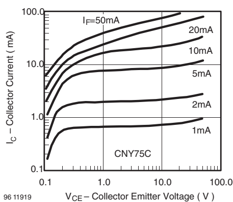
Figure 11. Collector Current vs. Collector Emitter Voltage
