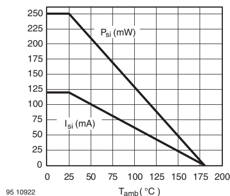
Figure 1. Derating diagram
