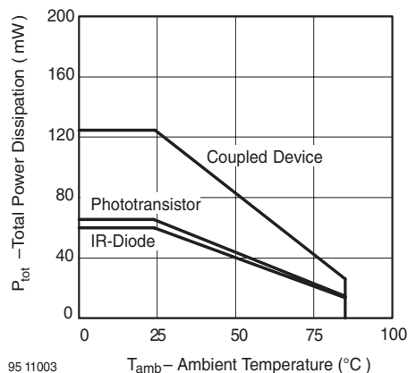
Figure 6. Total Power Dissipation vs. Ambient Temperature
