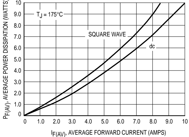
Figure 10. Power Dissipation
