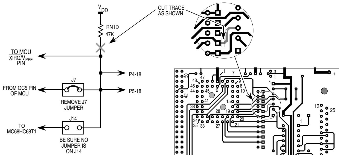
Figure 7. Isolating EVBU XIRQ Pin
