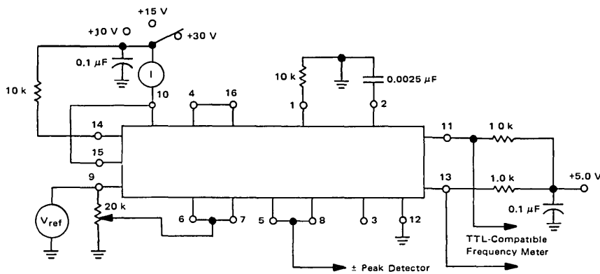
FIGURE 6 – FREQUENCY LIMIT TEST CIRCUIT
