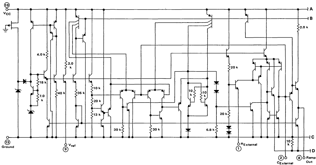
FIGURE 3 - CIRCUIT SCHEMATIC (continued next page)
