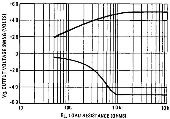
FIGURE 10 – OUTPUT VOLTAGE SWING versus LOAD RESISTANCE
