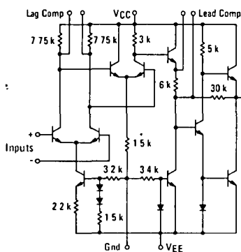
FIGURE 1 – MC1530/MC1430 (STANDARD INPUT)
