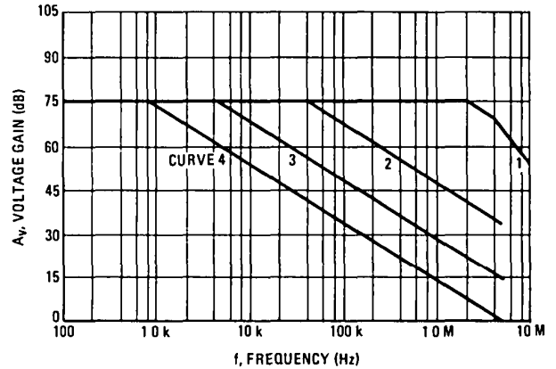
FIGURE 7 – MC1530/MC1430 OPEN LOOP VOLTAGE GAIN versus FREQUENCY
