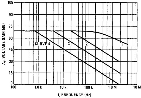
FIGURE 8 – MC1531/MC1431 OPEN LOOP VOLTAGE GAIN versus FREQUENCY
