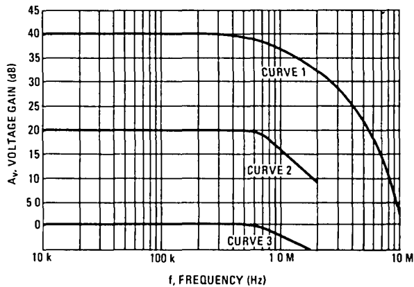
FIGURE 6 – MC1531/MC1431 VOLTAGE GAIN versus FREQUENCY
