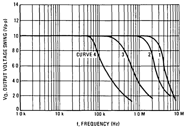
FIGURE 4 – LARGE SIGNAL SWING versus FREQUENCY
