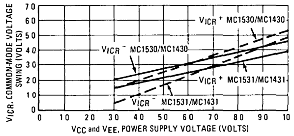
FIGURE 11 – COMMON-MODE SWING versus POWER SUPPLY VOLTAGE
