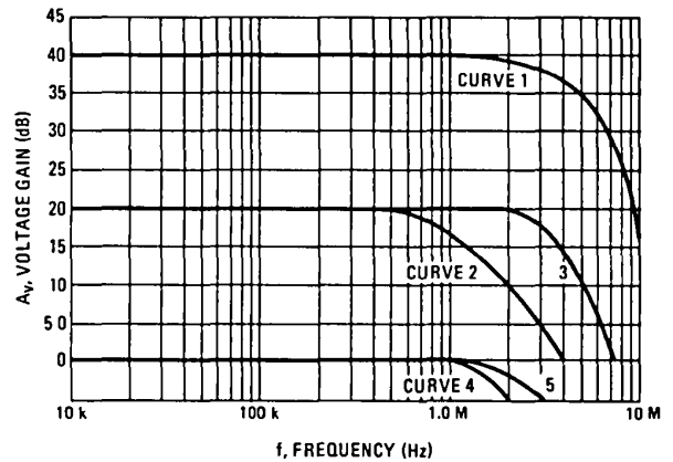
FIGURE 5 – MC1530/MC1430 VOLTAGE GAIN versus FREQUENCY
