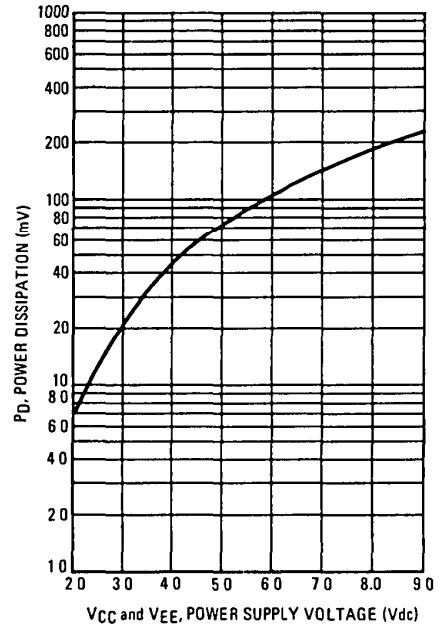
FIGURE 12 – POWER CONSUMPTION versus POWER SUPPLY VOLTAGE
