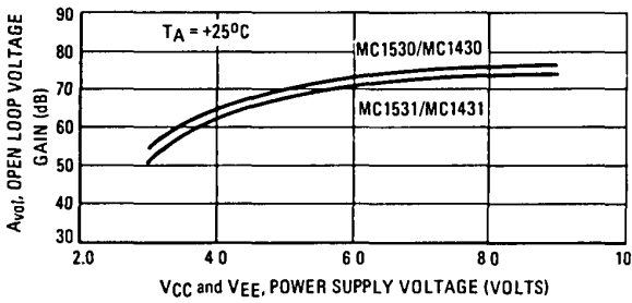
FIGURE 9 – VOLTAGE GAIN versus POWER SUPPLY VOLTAGE
