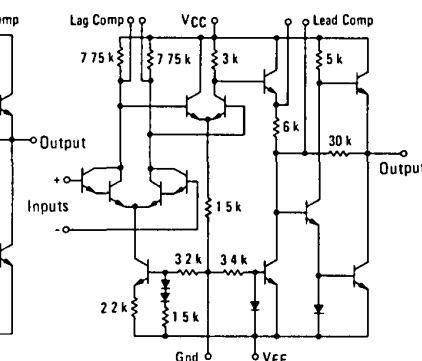
FIGURE 2 – MC1531/MC1431 (DARLINGTON INPUT)
