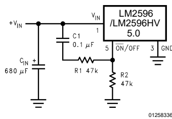
FIGURE 21. Delayed Startup
