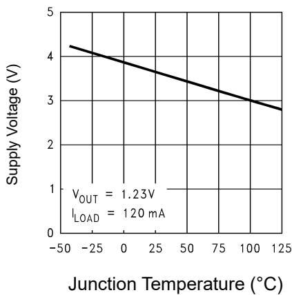
Figure 9: Supply Voltage
