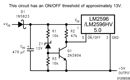
for Inverting Regulator FIGURE 23. Undervoltage Lockout
