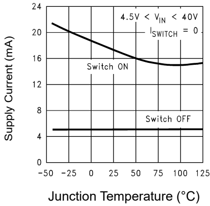
Figure 7: Quiescent Current
