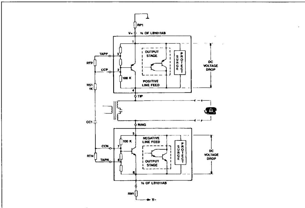
Figure 1 : Functional Diagram.
