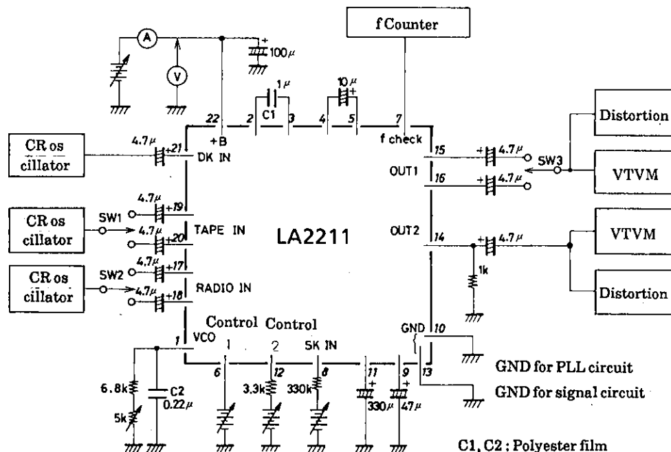
Fig. 1 Test Circuit
