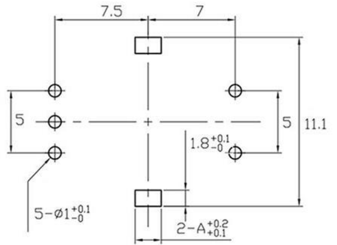
P.C.B.MOUNTING DETAIL
