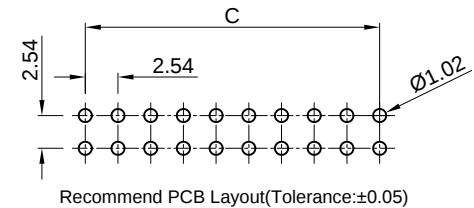
Recommend PCB Layout(Tolerance:±0.05)
