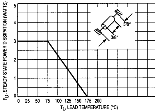
Figure 5. Steady State Power Derating
