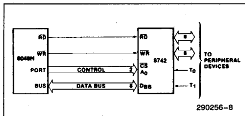
Figure 4. 8048H-8742 Interface
