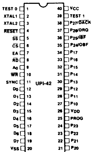
Figure 1. Pin Configuration
