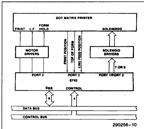
Figure 6. 8742 80-Column Matrix Printer Interface
