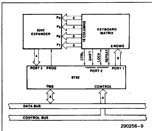
Figure 5. 8742-8243 Keyboard Scanner
