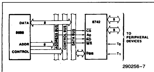
Figure 3. 8088-8742 Interface
