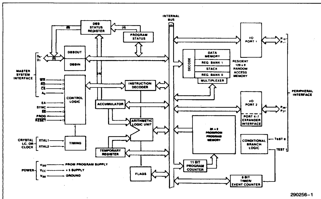
Figure 2. Block Diagram
