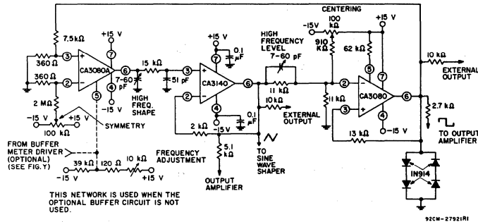
(a) Circuit
