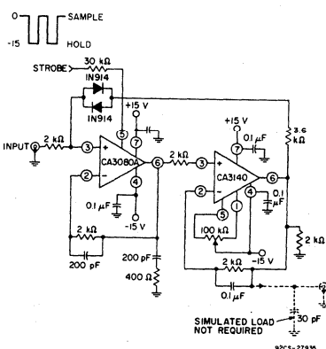
Fig. 34 — Sample-and-hold circuit.
