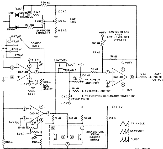
Fig. 24 - Sweeping generator.
