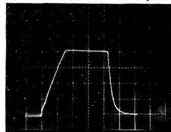
(a) SUPPLY TURN-ON AND TURN-OFF CHARACTERISTICS (5 VOLTS/DIV AND 1 s/DIV.) 92CS-27682
