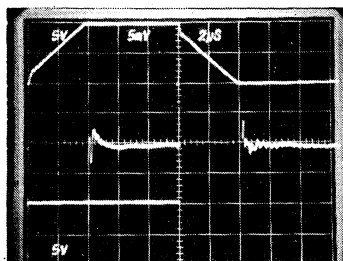
LARGE-SIGNAL RESPONSE AND SETTLING TIME TOP TRACE: OUTPUT SIGNAL (5 V/DIV. AND 2 \mu\text{s} /DIV.) BOTTOM TRACE: INPUT SIGNAL (5 V/DIV. AND 2 \mu\text{s} /DIV.) CENTER TRACE: DIFFERENCE OF INPUT AND OUTPUT SIGNALS THROUGH TEKTRONIX AMPLIFIER 7A13 (5 mV/DIV. AND 2 \mu\text{s} /DIV.)
