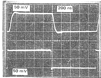
TOP TRACE: OUTPUT (50 mV/DIV AND 200 ns/DIV) BOTTOM TRACE: INPUT (50 mV/DIV AND 200 ns/DIV) (a) SMALL-SIGNAL RESPONSE (50 mV/DIV AND 200 ns/DIV)
