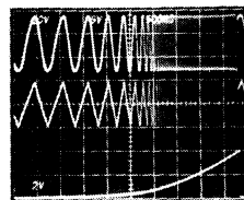
TOP TRACE: OUTPUT AT JUNCTION OF 2.7k AND 51k RESISTORS 5V/DIV AND 500ms/DIV CENTER TRACE: EXTERNAL OUTPUT OF TRIANGULAR FUNCTION GENERATOR 2V/DIV AND 500ms/DIV BOTTOM TRACE: OUTPUT OF "LOG" GENERATOR 10V/DIV AND 500ms/DIV
