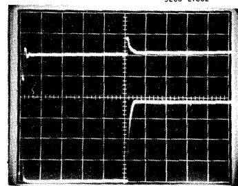
(b) TRANSIENT RESPONSE TOP TRACE: OUTPUT VOLTAGE (200 mV/DIV AND 5 μs/DIV) BOTTOM TRACE: COLLECTOR OF LOAD SWITCHING TRANSISTOR, LOAD = 1 AMPERE (5 VOLTS/DIV AND 5 μs/DIV) 92CS-27681
