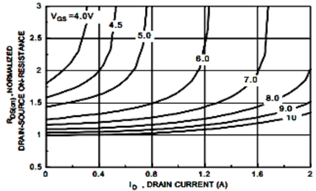
Fig 5: On-Resistance Variation with Drain Current and Temperature
