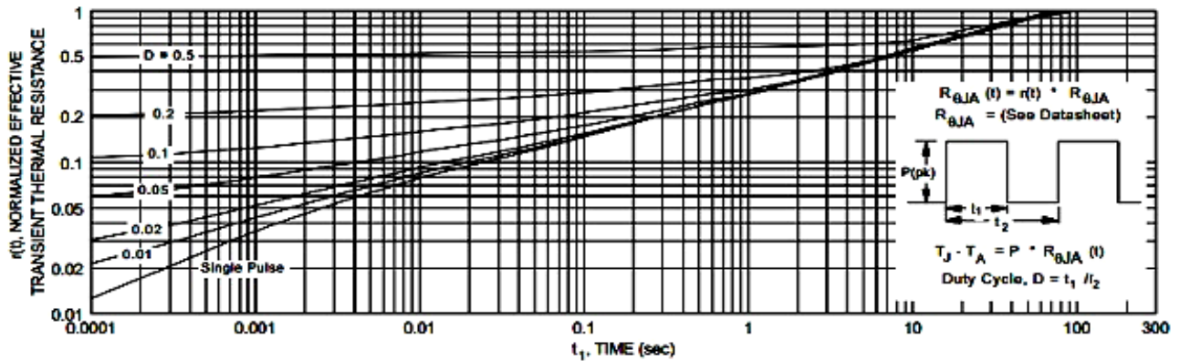
Fig 13: TO-92, BS170 Transient Thermal Response Curve
