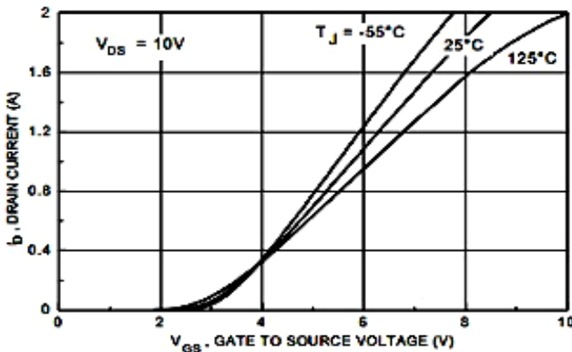
Fig 3: Transfer Characteristics
