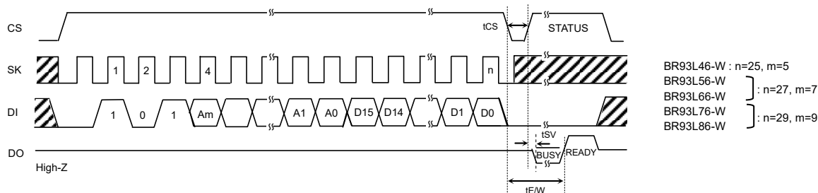
Figure 34. Write cycle
