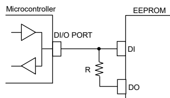
Figure 53. DI, DO control line common connection
