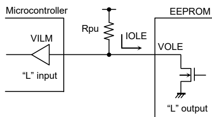
Figure 50. DO pull up resistance
