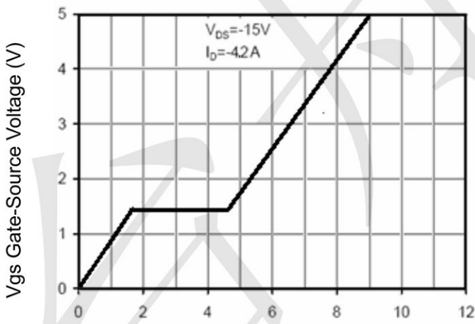
Figure 11 Gate Charge
