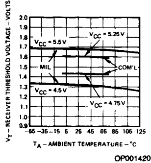
Am2908 Receiver Threshold Variation Versus Ambient Temperature
