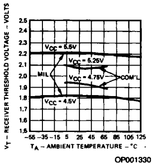
Am2907 Receiver Threshold Variation Versus Ambient Temperature
