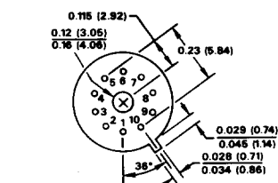
TO-100 "H"
