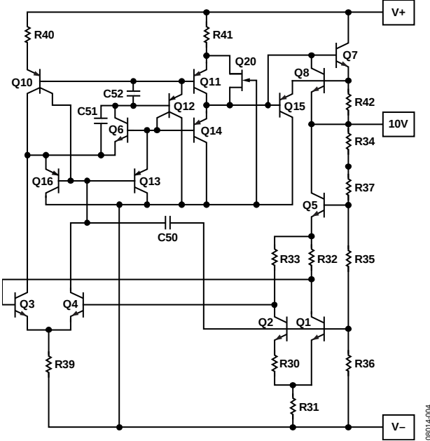
Figure 4. Simplified Schematic
