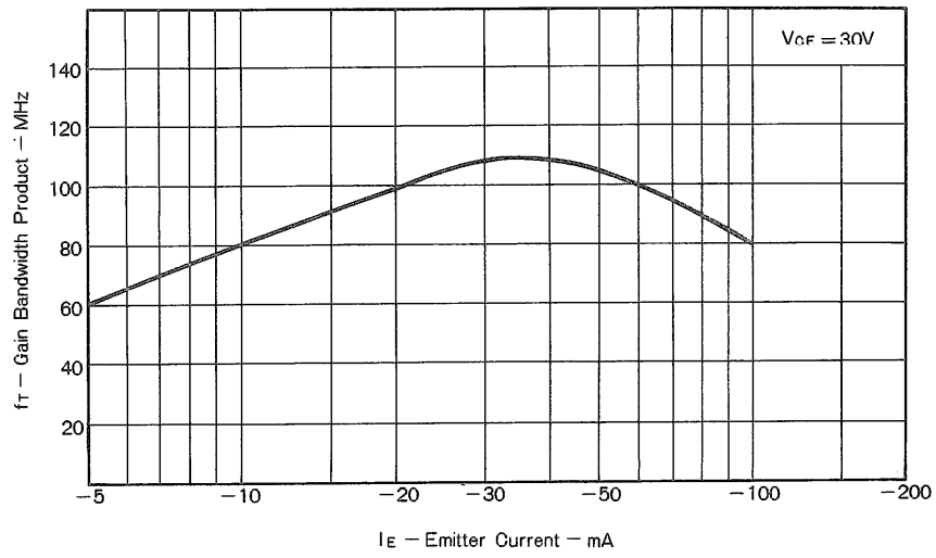
GAIN BANDWIDTH PRODUCT vs. EMITTER CURRENT
