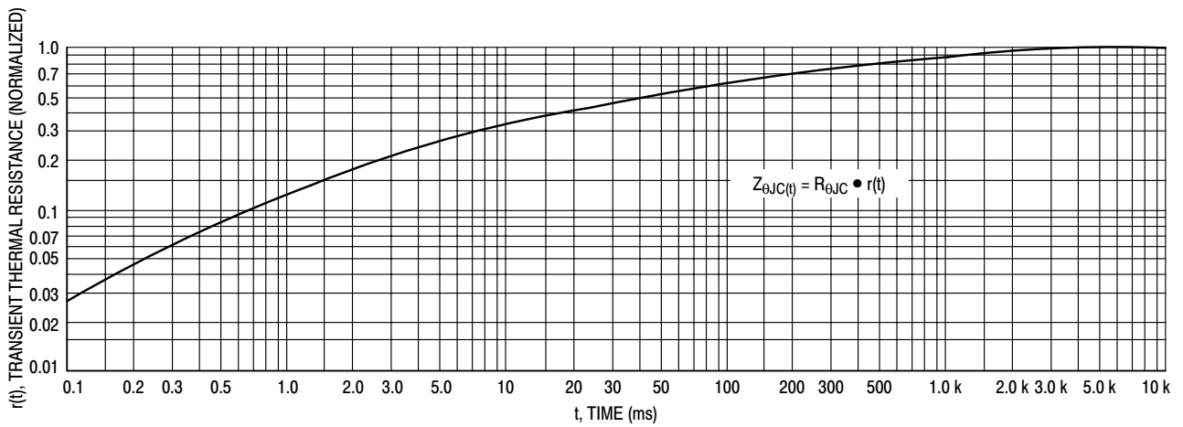
Figure 5. Thermal Response
