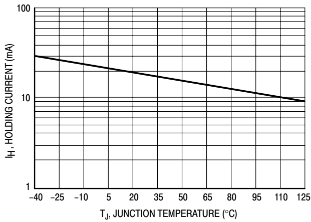
Figure 8. Typical Holding Current versus Junction Temperature
