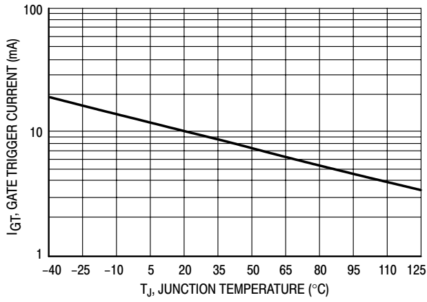
Figure 6. Typical Gate Trigger Current versus Junction Temperature
